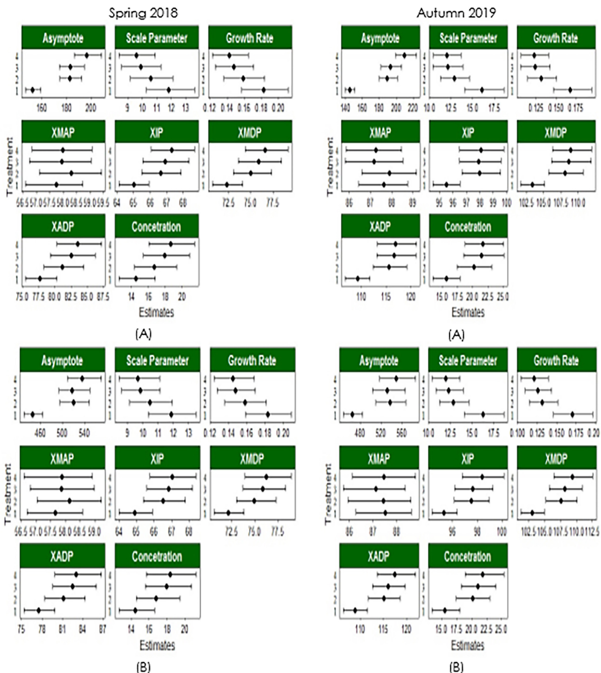
Figure 4 - Confidence intervals of parameters and critical points of the nonlinear logistic model estimated via bootstrap for mass of fruits (A) and number of fruits (B), asymptote ( \mu ), scale parameter ( k ), growth rate ( r ), and XMAP (point of maximum acceleration).
